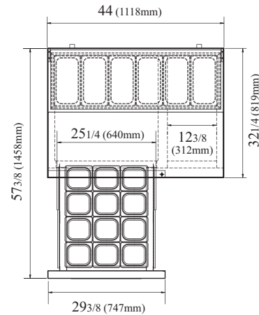
PLAN VIEW
